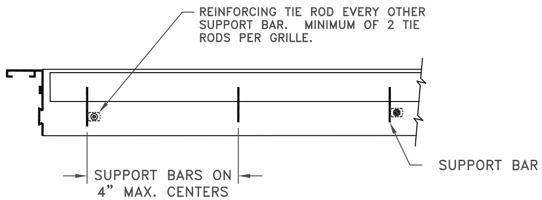
'L' SERIES GRILLE REINFORCED FOR FLOOR USE
