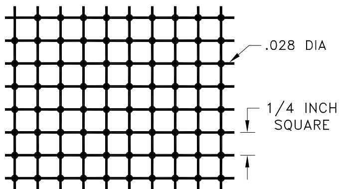
WGH4 1/4 INCH GALVANIZED HARDWARE CLOTH
