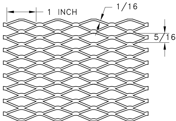
WBS ALUMINUM BIRD SCREEN FINISHED THICKNESS .031
