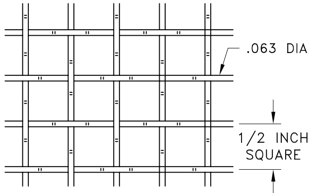
WAMIC WOVEN ALUMINUM MESH INTER CRIMPED
