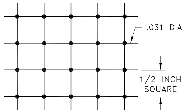
WGH2 1/2 INCH GALVANIZED HARDWARE CLOTH
