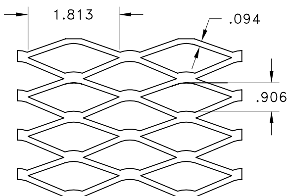
WBS-1 ALUMINUM BIRD SCREEN FINISHED THICKNESS .050
