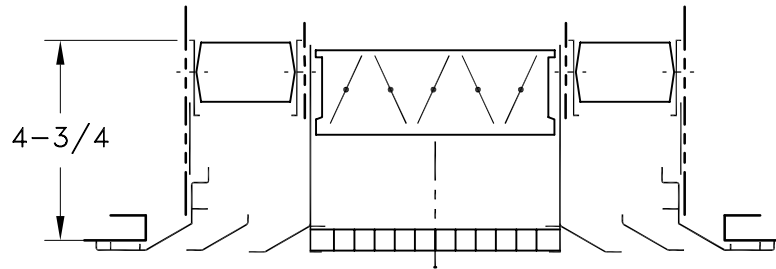
DIFFUSER WITH OPTIONAL O.B. SUPPLY AND O.B. RETURN DAMPER
