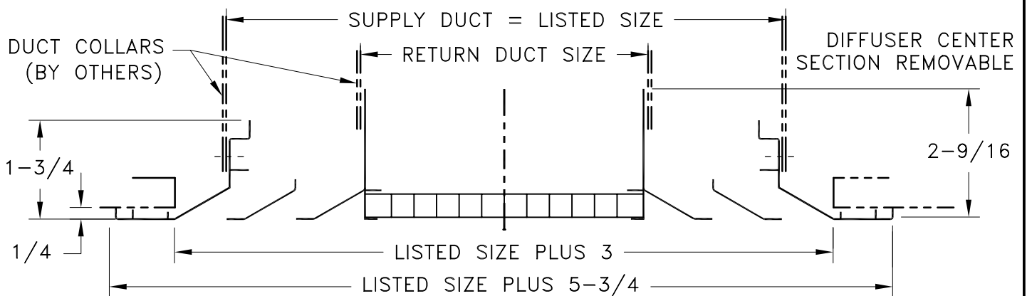
DETAIL OF OPTIONAL LEAF SUPPLY DAMPER WHEN RETURN DUCT SIZE IS 3 INCHES LESS THAN SUPPLY DUCT SIZE
