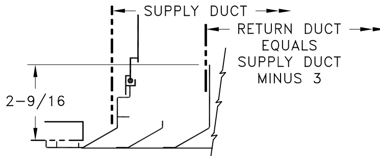
DETAIL OF OPTIONAL LEAF SUPPLY DAMPER WHEN RETURN DUCT SIZE IS 3 INCHES LESS THAN SUPPLY DUCT SIZE
